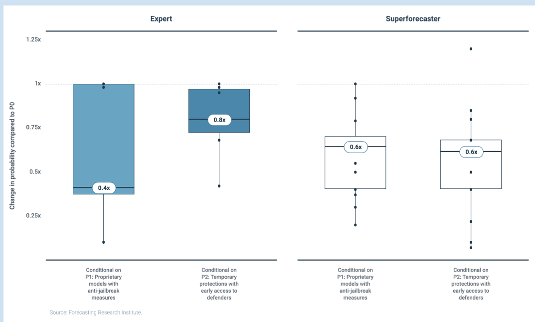
Figure ES5. Survey results on the effect of different risk management policies on the risk of data-damaging worms, conditional on AI Elite Exploit Uplift.
