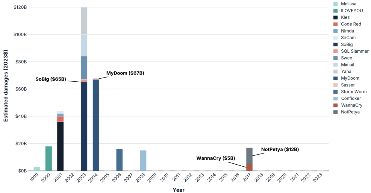
Figure A.2. Damages from major worm attacks in Johansmeyer dataset (1999–2023)
