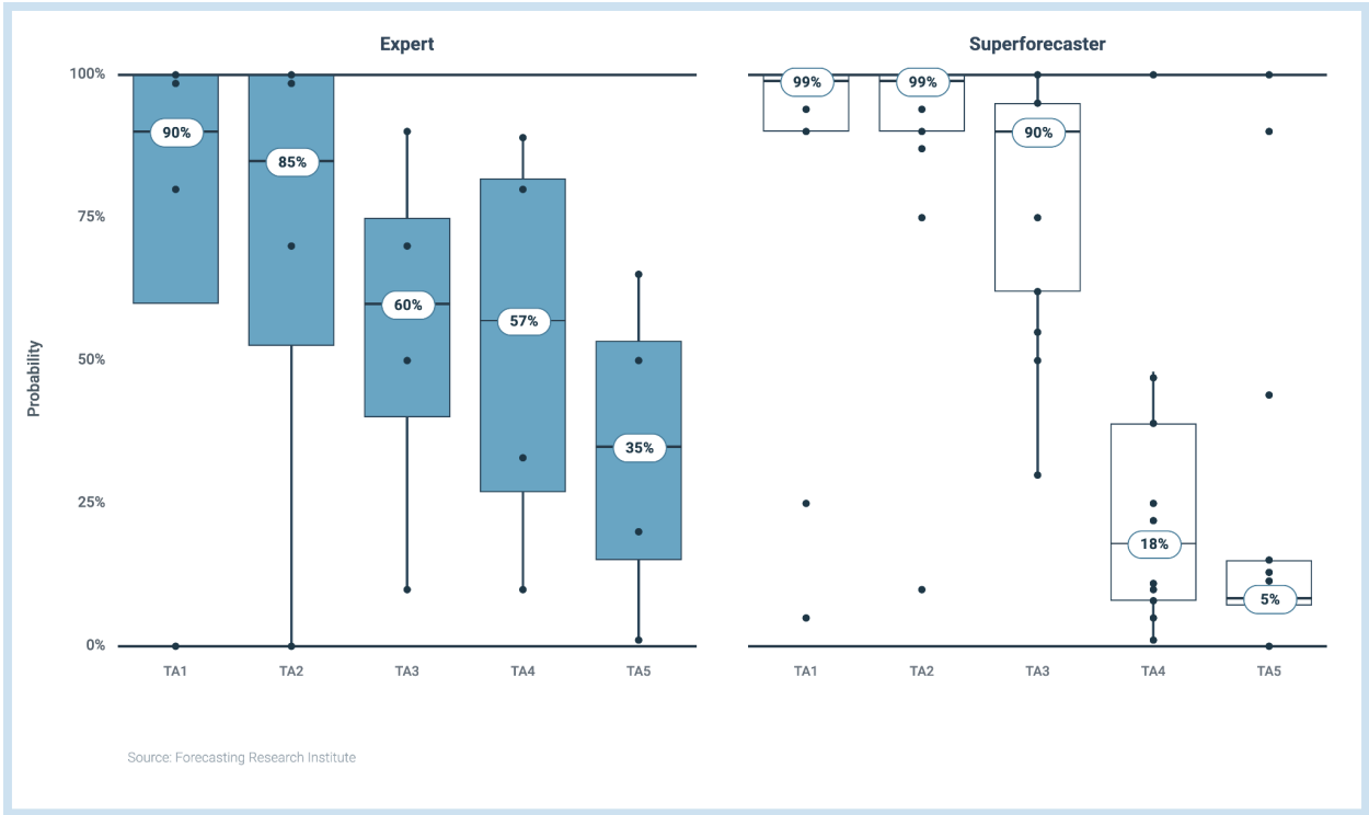
Figure 2.2. Expert and superforecaster estimates of the probability that at least one actor in each threat actor class would be willing, over a year, to launch a data-damaging worm attack if they were capable. 34
