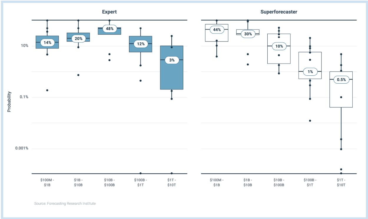
Figure 6.8: The probability of data-damaging worm attacks causing different amounts of economic damages in 2026, conditional on Elite Exploit Uplift
