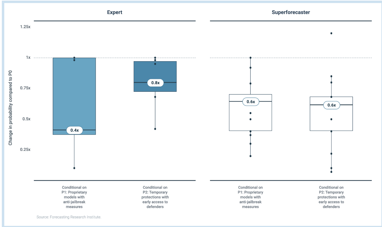
Figure 6.11. Relative risk of a >$10B data-damaging worm attack compared to P0, conditional on AI elite exploit uplift.
